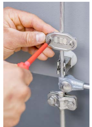
Fourth step: Fix the marked number plate at the down conductor.
