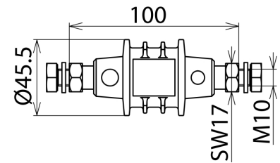
Dimension drawing EXFS 100
