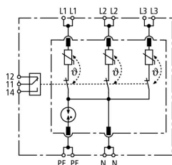
Basic circuit diagram DR M 4P 255 FM
