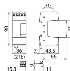
Dimension drawing DR M 4P 255 SN1872 FM
