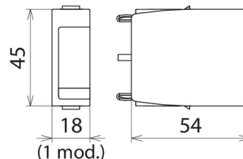
Dimension drawing DG MOD ACI 275
