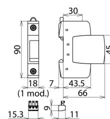
Dimension drawing DG S 48 FM
