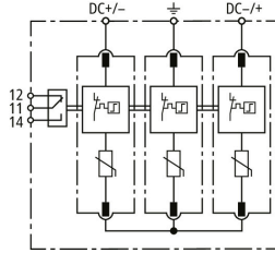
Basic circuit diagram DG M YPV 1200 FM - old
