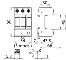
Dimension drawing DG M YPV 1200 FM - old
