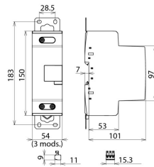
Dimension drawing DBM 1 CI 440 FM
