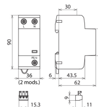
Dimension drawing DSH TN 255 FM
